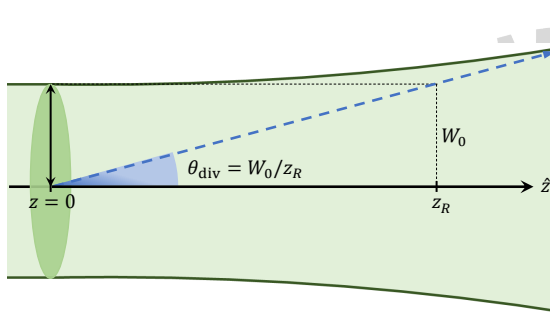
Figure 2.4 : Illustration of the beam-radius evolution and far-field divergence angle \theta_{\text{div}} .
