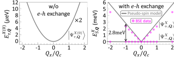
Figure 1.4 : The lowest valley-degenerate (left) and valley-split (right) exciton bands in MoS 2 along the Q_x direction, reproduced from Ref. [7].
