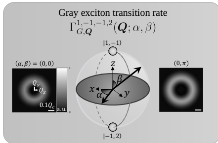
Figure 3.7 : Normalized transition rate of GXs excited by a VVB state |1, -1, -1, 2; \alpha, \beta\rangle in momentum space at the north/south poles of the Poincaré sphere.
