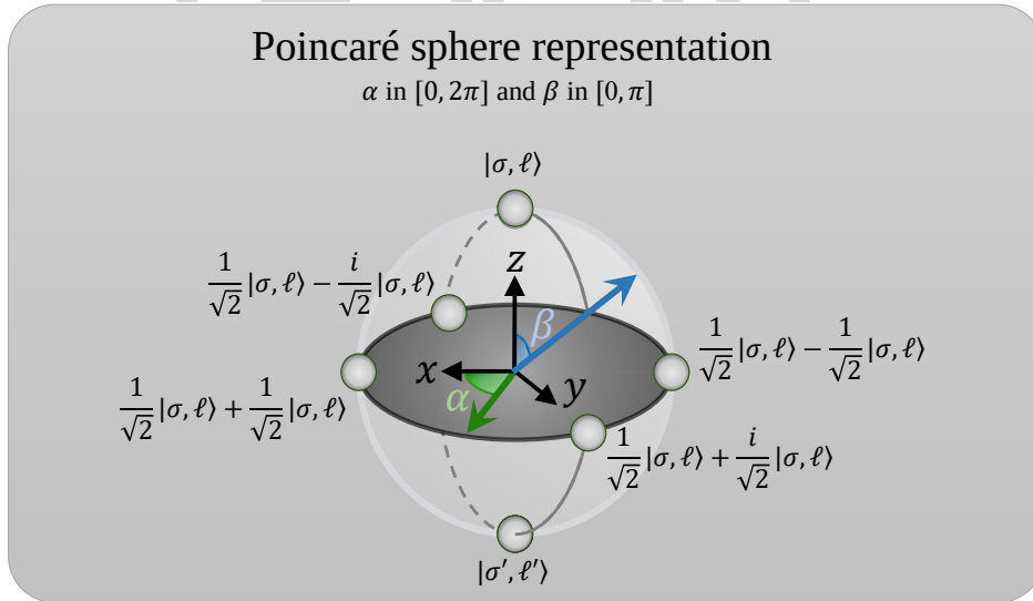
Figure 2.5 : Representation of a VVB state on the Poincaré sphere, parameterized by the azimuthal angle \alpha and polar angle \beta . Several representative combinations of \alpha and \beta are illustrated on the sphere surface as examples.
