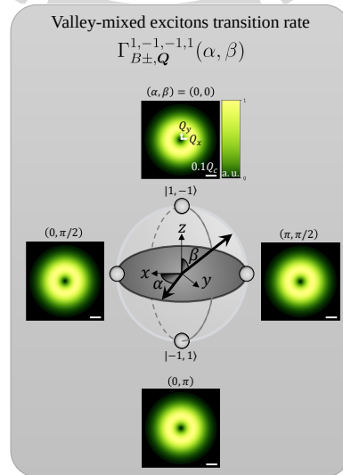
Figure 3.3 : Normalized transition rate of total BXs excited by a VVB state |1, -1, -1, 1; \alpha, \beta\rangle in momentum space.
