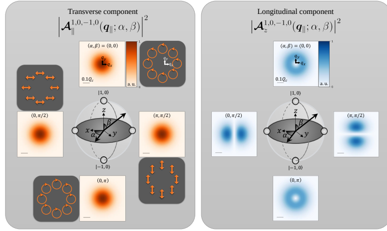
Figure 2.6 : Angular-spectrum distribution (squared magnitude) of different components of \mathcal{A}_{\parallel}^{1,0,-1,0}(\mathbf{q}_{\parallel}; \alpha, \beta) on the Poincaré sphere, together with the corresponding polarization states of the transverse components.
