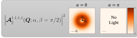
Figure 3.4 : Distribution of the transverse component for a VVB state |1, 1, 1, 1; \alpha, \beta\rangle in momentum space.
