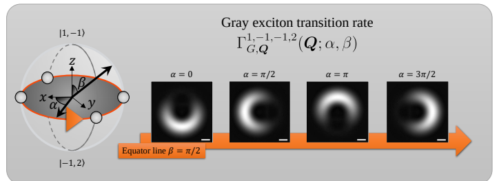
Figure 3.8 : Normalized transition rate of GXs excited by a VVB state |1, -1, -1, 2; \alpha, \beta\rangle in momentum space along the equator of the Poincaré sphere. The scale and color bars are the same as in Fig. 3.7.
