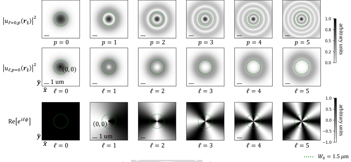
Figure 2.1 : Squared magnitude (intensity) and phase distribution of u_{\ell,p}(\mathbf{r}_{\parallel}) . The green dotted line denotes the beam waist W_0 . The scale bar indicates the length of 1 \mu\text{m}
