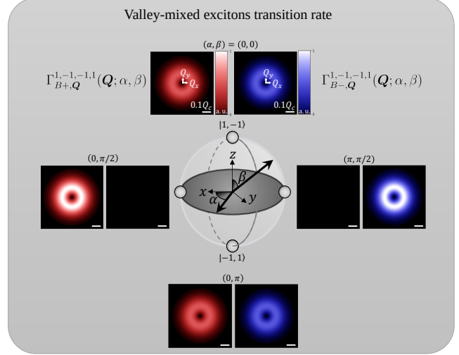
Figure 3.2 : Normalized transition rate of valley-mixed BXs excited by a VVB state |1, -1, -1, 1; \alpha, \beta\rangle in momentum space.
