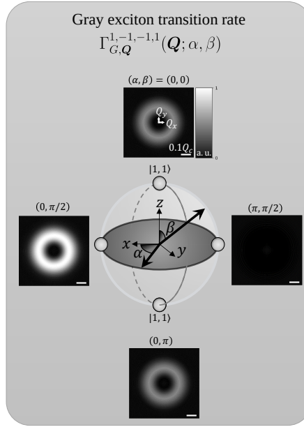
Figure 3.6 : Normalized transition rate of GXs excited by a VVB state |1, -1, -1, 1; \alpha, \beta\rangle in momentum space.
