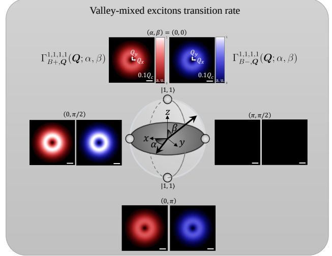
Figure 3.5 : Normalized transition rate of valley-mixed BXs excited by a VVB state |1, 1, 1, 1; \alpha, \beta\rangle in momentum space.
