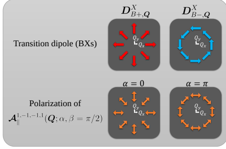
Figure 3.1 : Illustration of the transition dipole moments of valley-mixed BXs, reproduced from [6], and their matching with the transverse polarization of a VVB state |1, -1, -1, 1; \alpha, \beta\rangle in momentum space.
