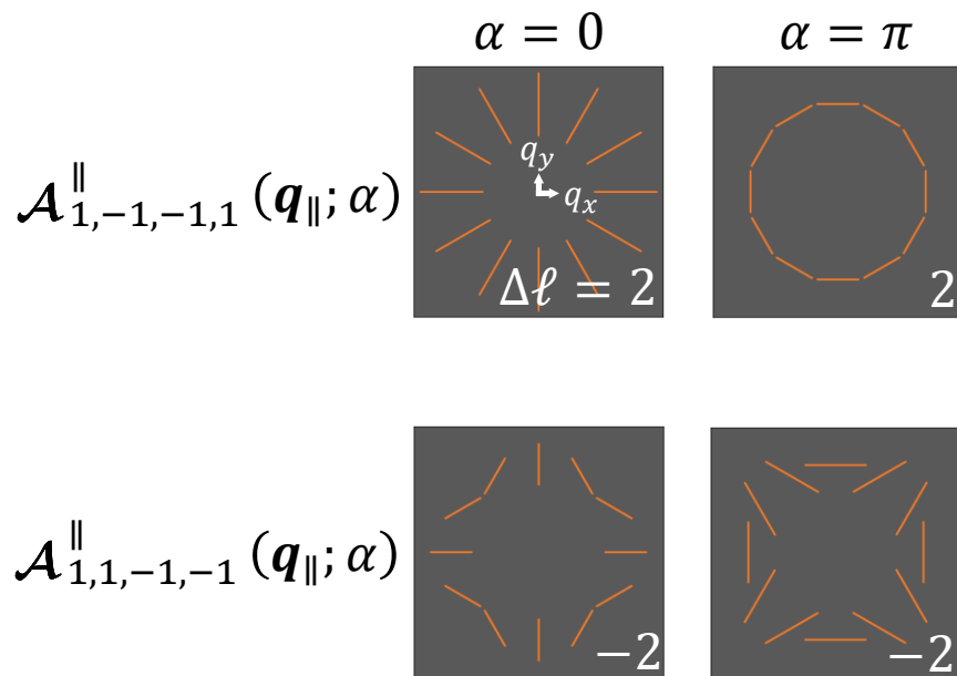
Polarization trajectory
