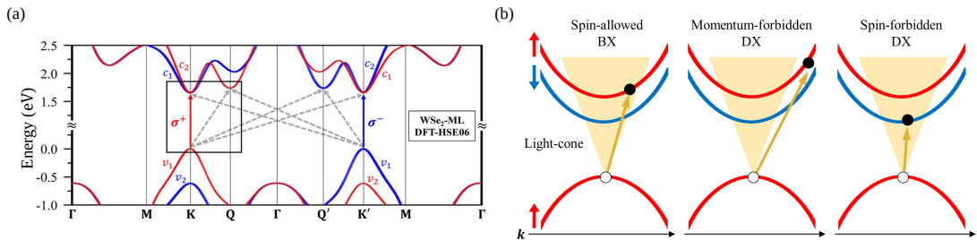
Figure 1.3 : (a) Calculated band structure of \text{WSe}_2 , showing spin-up (red) and spin-down (blue) states, together with a schematic illustration of valley-selective optical transitions at the K and K' valleys, which couple to right- and left-circularly polarized light, respectively, reproduced from Ref. [5]. (b) Schematic configurations of excitonic states, including spin-allowed bright excitons (BXs), momentum-forbidden dark excitons (DXs), and spin-forbidden DXs.
