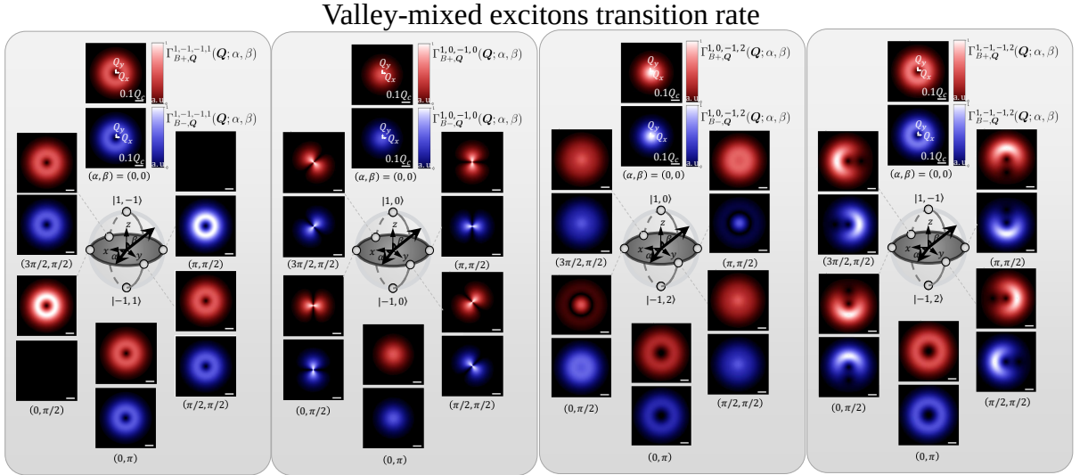
Figure 3.2 : Normalized transition rate of valley-mixed BXs excited by the VVB state |1, \ell, -1, \ell'; \alpha, \beta\rangle in center of mass momentum space. The scale bar indicates the considered 0.1 times light cone range for WSe 2 -monolayers, Q_c = 8.6 \mu\text{m}^{-1}
