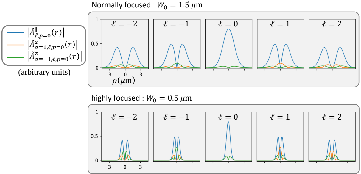
Figure 2.5 : Magnitude (absolute value) of \mathbf{A}_{\sigma,\ell,p=0}(\mathbf{r}) at z = 0 for different components and spin. The \sigma\ell term leads to asymmetry between cases with the same \ell in the longitudinal component (a wavelength of 532 nm is assumed).
