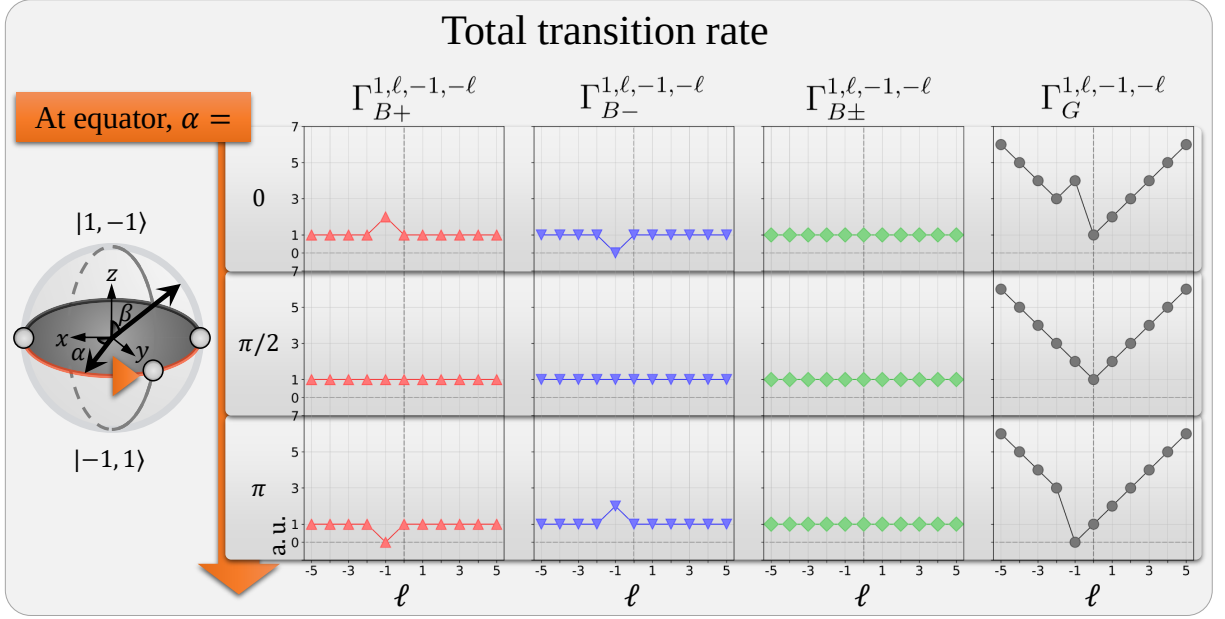
Figure 3.4 : Normalized total transition rates of BXs, total BXs, and GX excited by a VVB state |1, \ell, -1, -\ell; \alpha, \beta = \pi/2\rangle , for \ell \in \mathbb{Z} with \ell \in [-5, 5] , and for azimuthal angles \alpha = 0, \pi/2, \pi .
