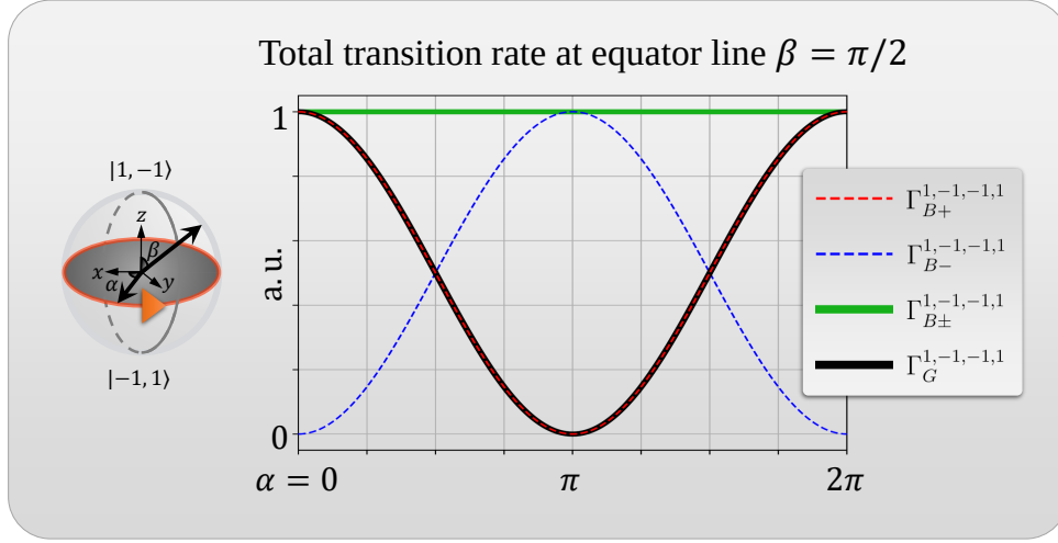
Figure 3.5 : Normalized total transition rates of BXs, total BXs, and GXs excited by a VVB state |1, -1, -1, 1; \alpha, \beta = \pi/2\rangle for azimuthal angles \alpha = 0 to 2\pi .
