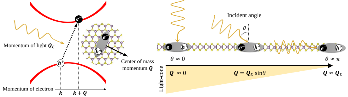
Figure 1.2 : Illustration of a photon carrying momentum Q_c exciting (leaving) an electron (hole) with momentum k + Q ( -k ), forming an exciton with center-of-mass (COM) momentum Q . Schematic of ideal of light cone and relation between COM momentum Q and Q_c
