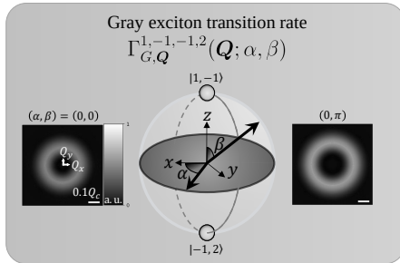
Figure 3.7 : Normalized transition rate of GXs excited by the VVB state |1, -1, -1, 2; \alpha, \beta\rangle in momentum space at the north/south poles of the Poincaré sphere.
