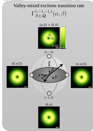
Figure 3.3 : Normalized transition rate of total BXs excited by the VVB state |1, -1, -1, 1; \alpha, \beta\rangle in momentum space.
