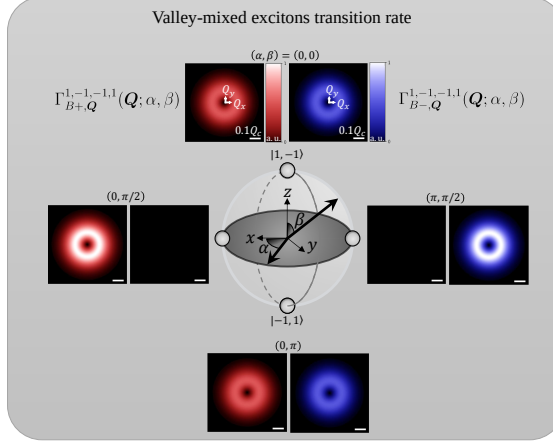
Figure 3.2 : Normalized transition rate of valley-mixed BXs excited by the VVB state |1, -1, -1, 1; \alpha, \beta\rangle in momentum space.
