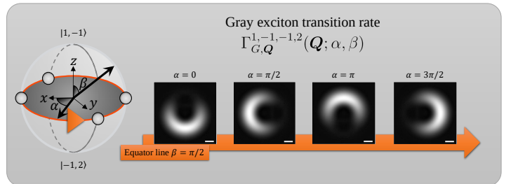
Figure 3.8 : Normalized transition rate of GXs excited by the VVB state |1, -1, -1, 2; \alpha, \beta\rangle in momentum space along the equator of the Poincaré sphere. The scale and color bars are the same as in Figure 3.7.
