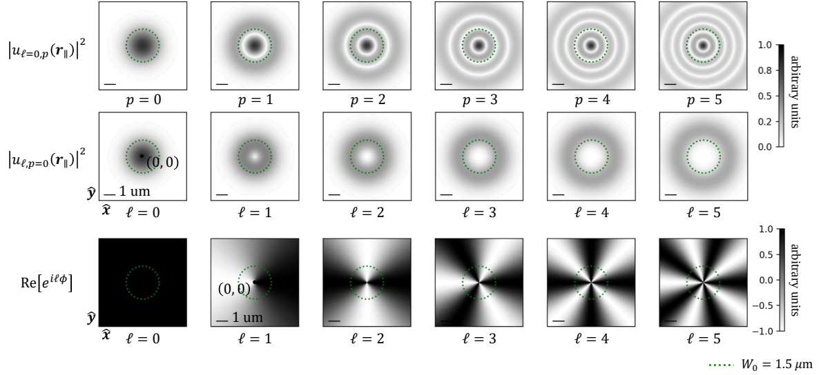
Figure 2.1 : Squared magnitude (intensity) and phase distribution of u_{\ell,p}(\mathbf{r}_{\parallel}) at z = 0 . The green dotted line denotes the beam waist W_0 . The scale bar indicates the length of 1 \mu\text{m} .
