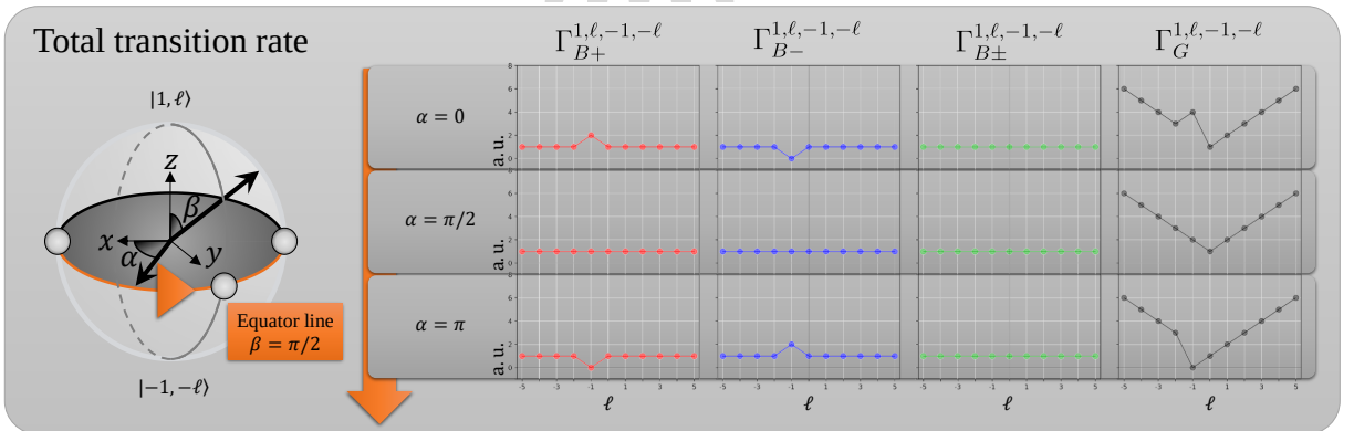
Figure 3.9 : Normalized total transition rates of BXs, total BXs, and GX excited by a VVB state |1, \ell, -1, -\ell; \alpha, \beta = \pi/2\rangle , for \ell \in \mathbb{Z} with \ell \in [-5, 5] , and for azimuthal angles \alpha = 0, \pi/2, \pi .
