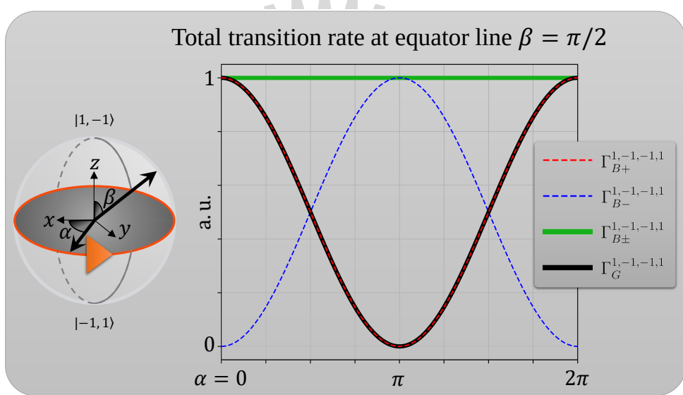
Figure 3.10 : Normalized total transition rates of BXs, total BXs, and GXs excited by a VVB state |1, -1, -1, 1; \alpha, \beta = \pi/2\rangle for azimuthal angles \alpha = 0 to 2\pi .
