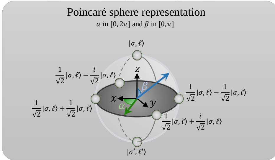
Figure 2.5 : The VVB state represented on the Poincaré sphere, parameterized by the azimuthal angle \alpha and polar angle \beta . Several representative combinations of \alpha and \beta are illustrated on the sphere surface as examples.
