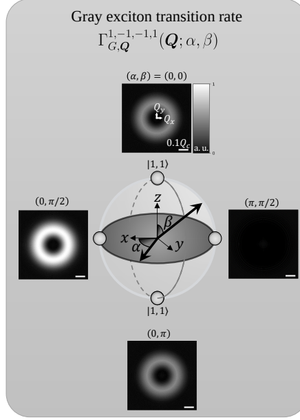
Figure 3.6 : Normalized transition rate of GXs excited by the VVB state |1, -1, -1, 1; \alpha, \beta\rangle in momentum space.
