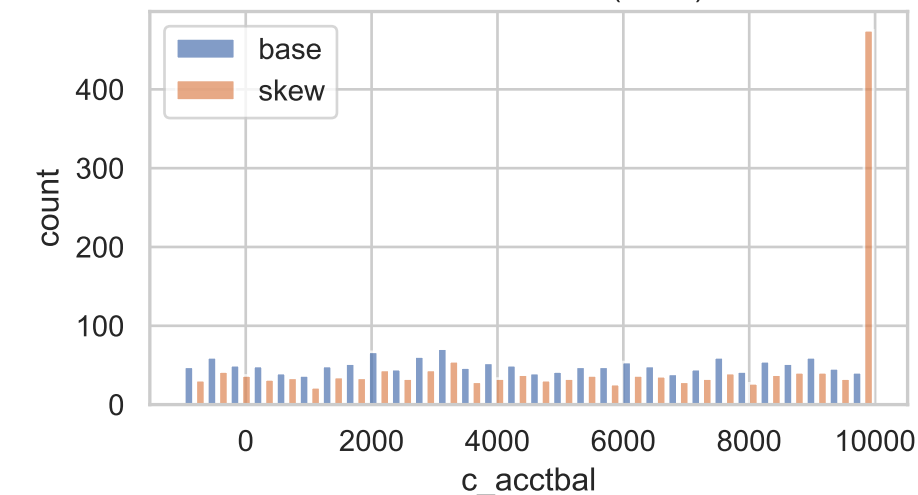
Customer acctbal (skew)
