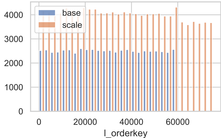
Lineitem order key (l_orderkey): base vs scale
