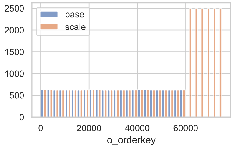
Orders key (o_orderkey): base vs scale
