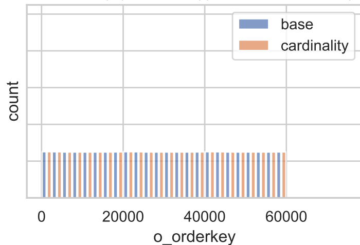
Orders key (o_orderkey): base vs cardinality
