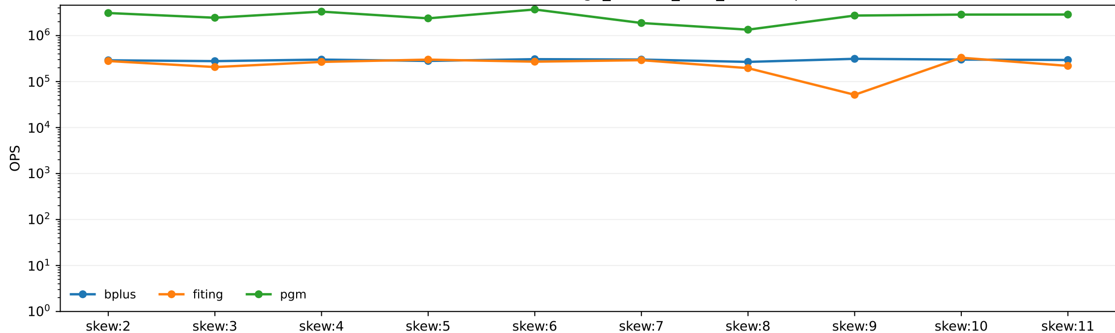
OPS vs data (skew, workload=range_uniform_r100_10000, op=scan)
