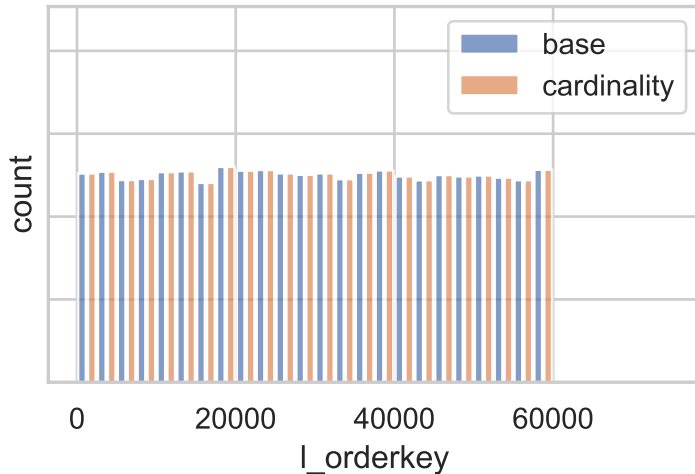
Lineitem -&gt; Orders (l_orderkey): base vs cardinality
