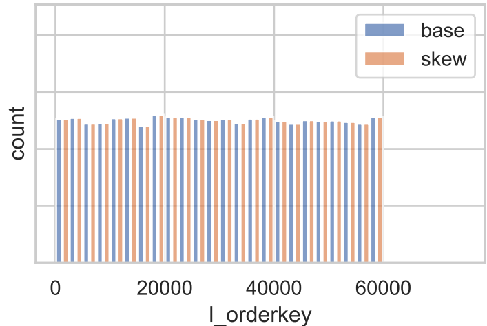
Lineitem -&gt; Orders (l_orderkey): base vs skew
