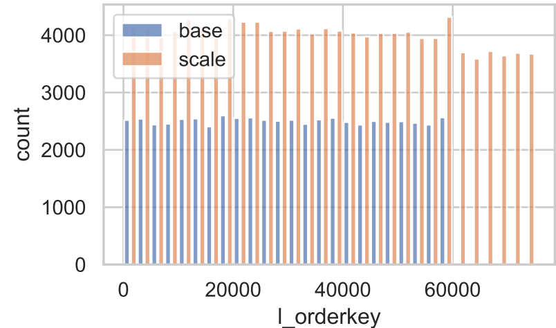
Lineitem -&gt; Orders (l_orderkey): base vs scale
