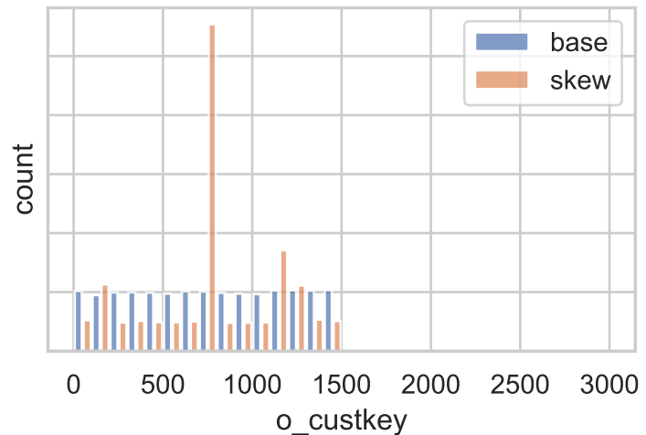
Orders -> Customer (o_custkey): base vs skew
