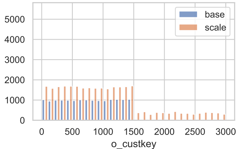
Orders -> Customer (o_custkey): base vs scale
