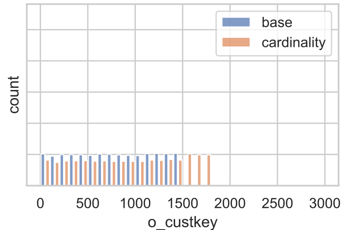
Orders -> Customer (o_custkey): base vs cardinality
