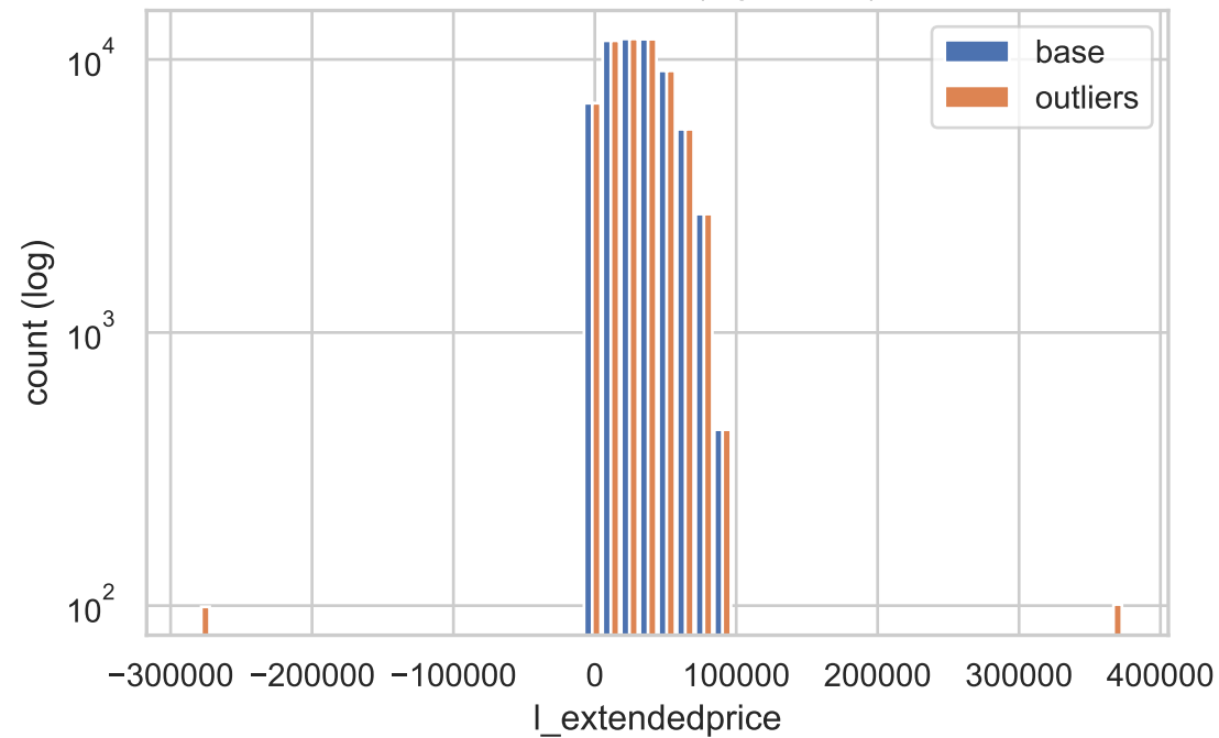
l_extendedprice (log-counts)
