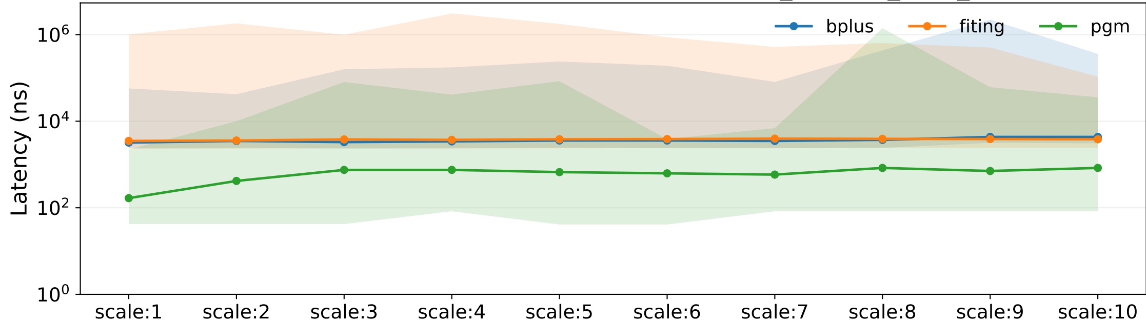
Latency p50/min/max vs data (cardinality, workload=range_uniform_r100_10000, op=scan)
