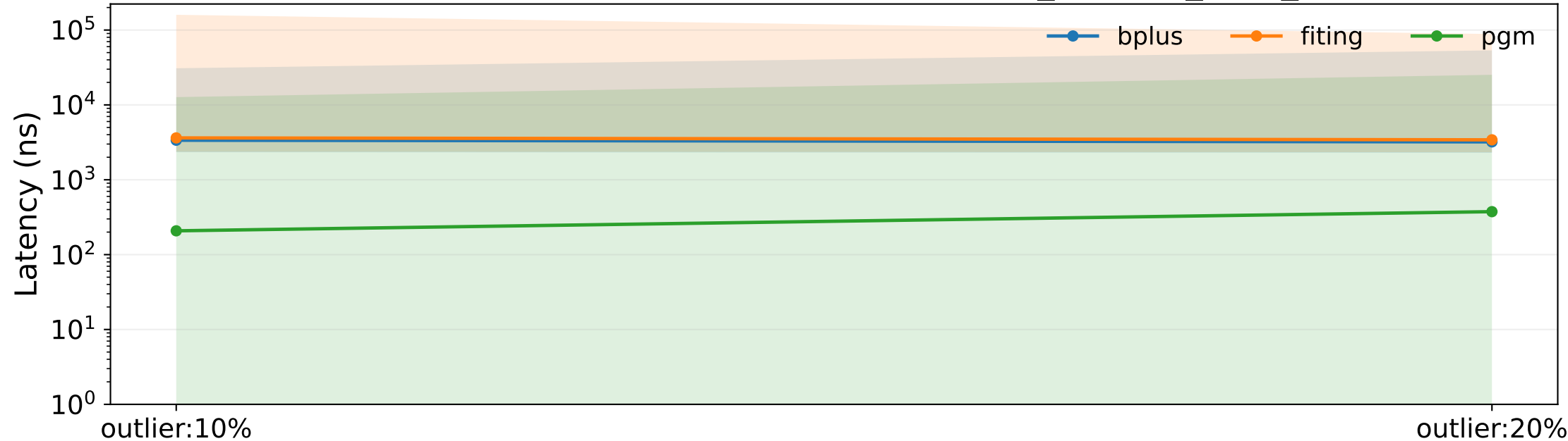
Latency p50/min/max vs data (outliers, workload=range_uniform_r100_10000, op=scan)
