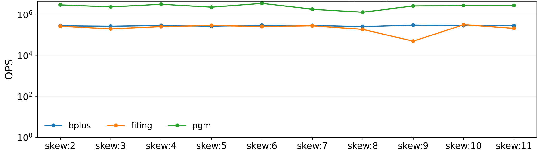
OPS vs data (skew, workload=range_uniform_r100_10000, op=scan)
