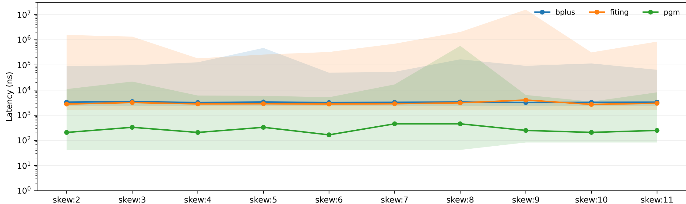
Latency p50/min/max vs data (skew, workload=range_uniform_r100_10000, op=scan)
