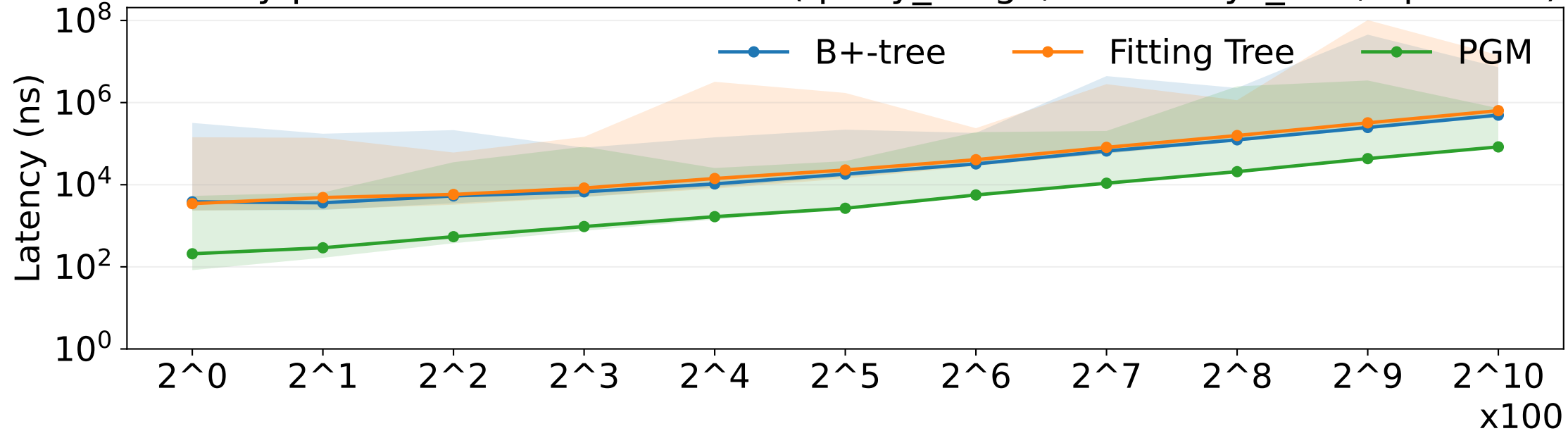
Latency p50/min/max vs workload (query_range, data=keys_u64, op=scan)
