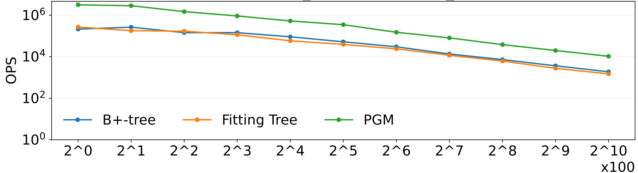
OPS vs workload (query_range, data=keys_u64, op=scan)
