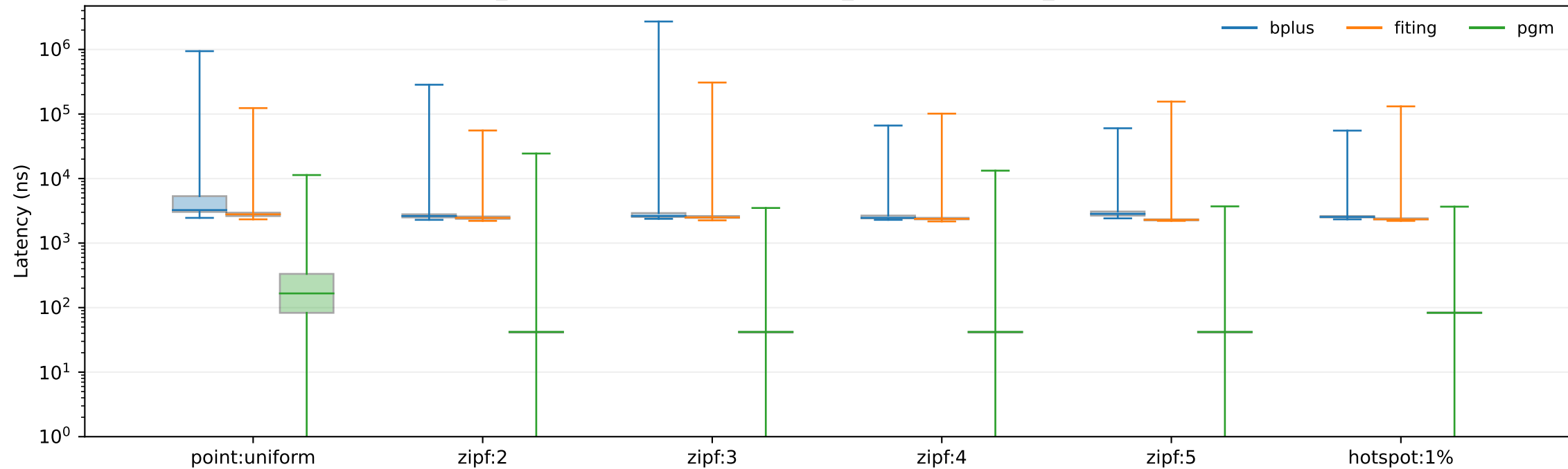
latency_ns boxplot vs workload (query_point, data=keys_u64, op=lookup)
