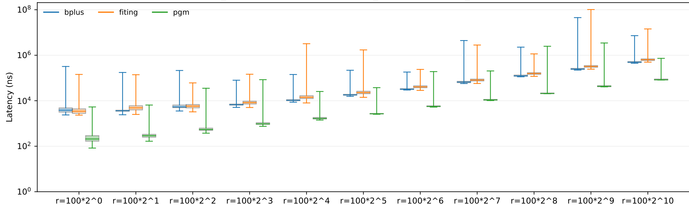
latency_ns boxplot vs workload (query_range, data=keys_u64, op=scan)
