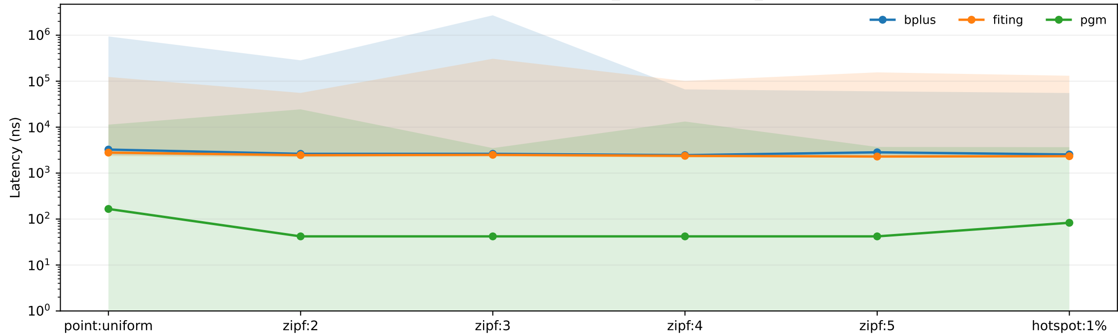
Latency p50/min/max vs workload (query_point, data=keys_u64, op=lookup)
