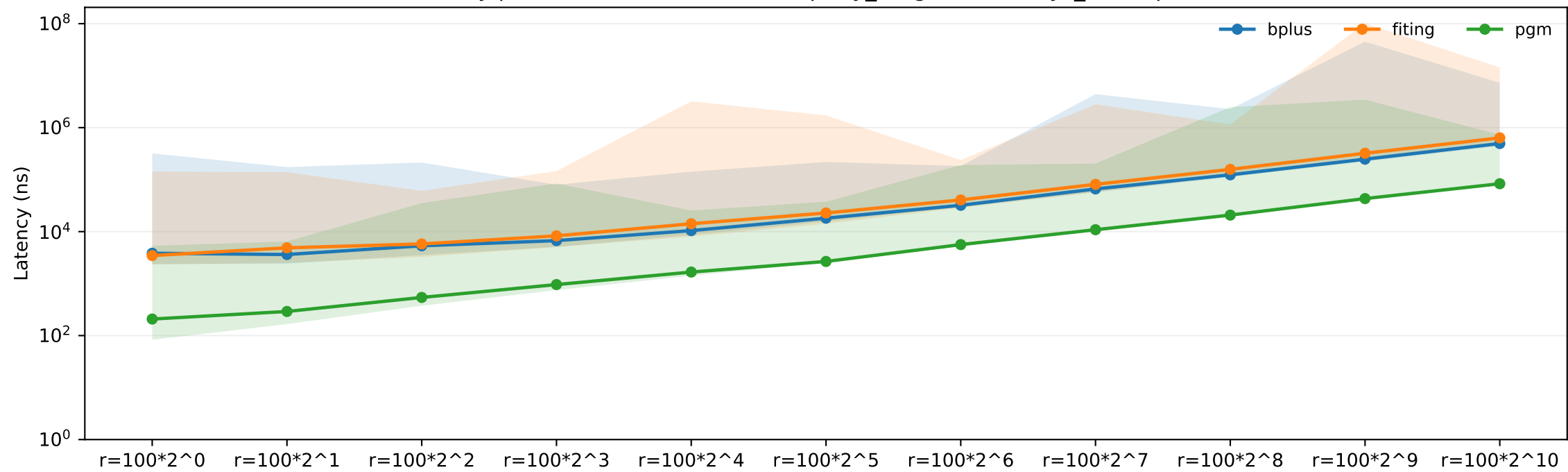
Latency p50/min/max vs workload (query_range, data=keys_u64, op=scan)
