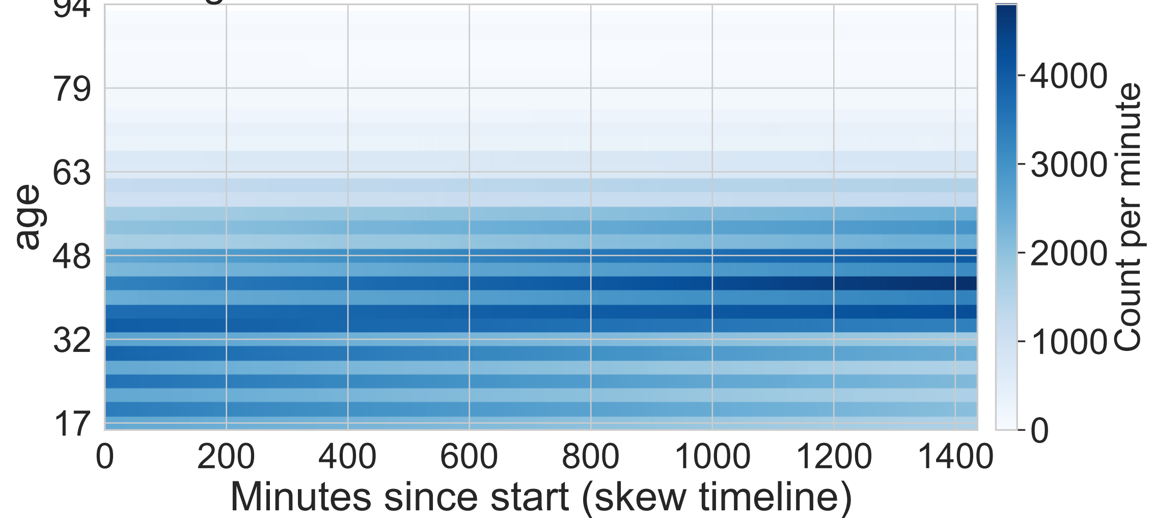
age distribution transition: base \rightarrow skew
