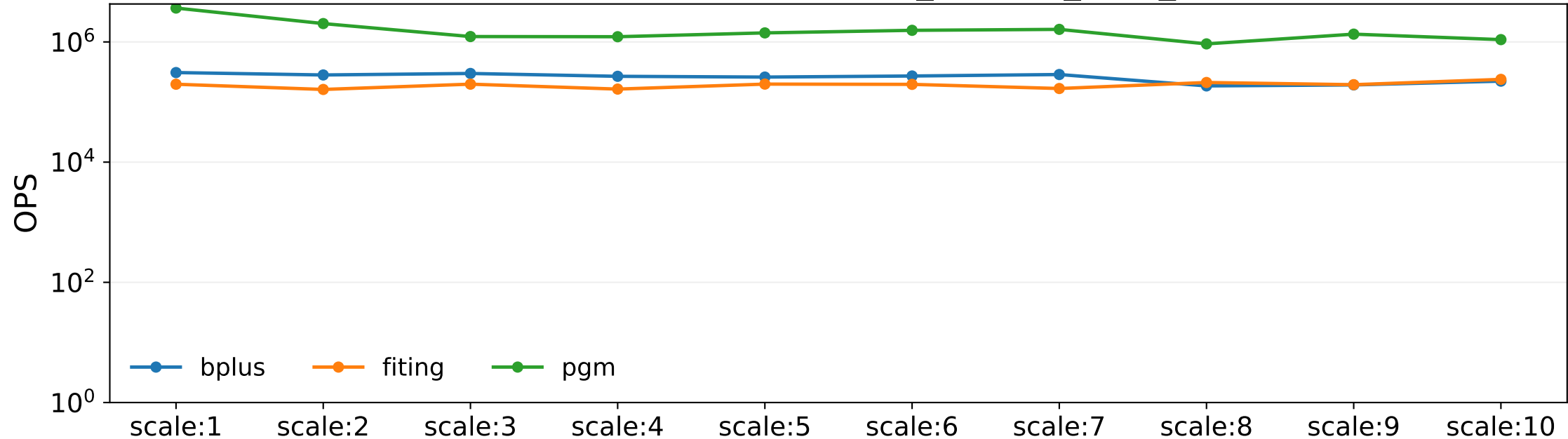
OPS vs data (cardinality, workload=range_uniform_r100_10000, op=scan)
