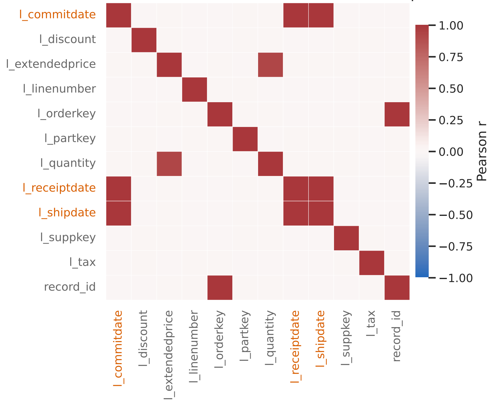
TPC-H SF16 (lineitem) – correlation heatmap
