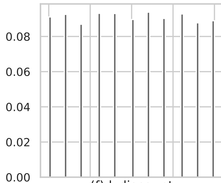
(f) l_discount
