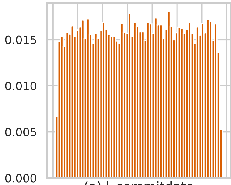
(a) l_commitdate
