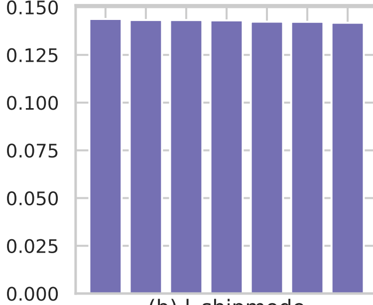
(b) l_shipmode
