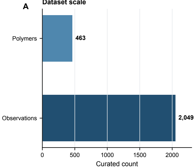
Dataset scale
