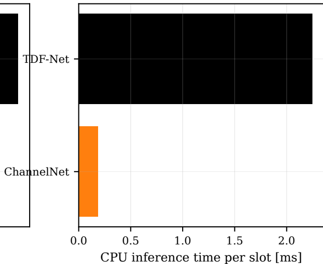
(b) inference cost
