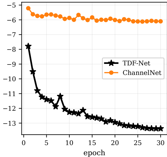
(b) validation loss
