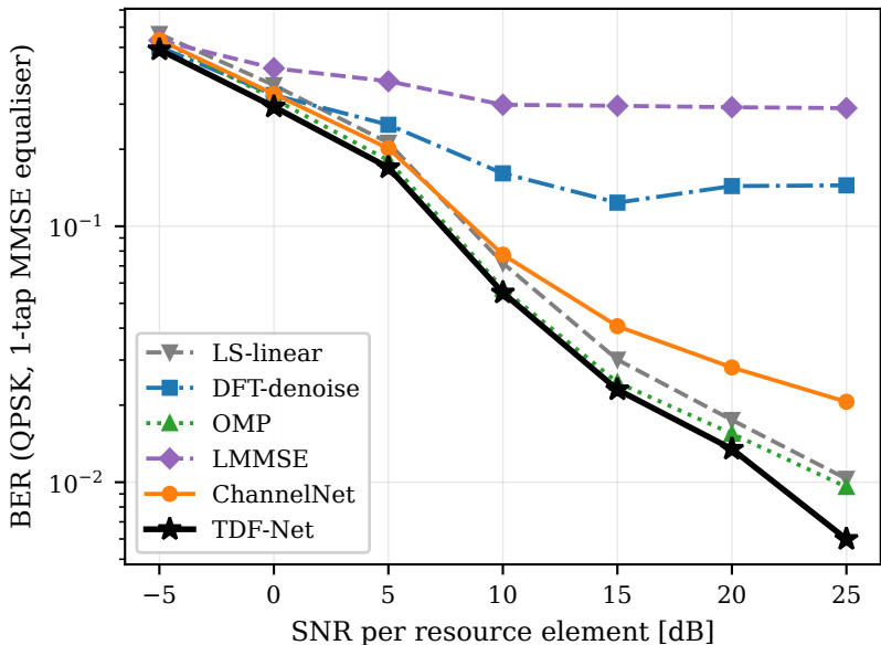
TDL-C, v = 100 km/h
