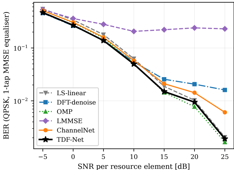
TDL-C, v = 30 km/h
