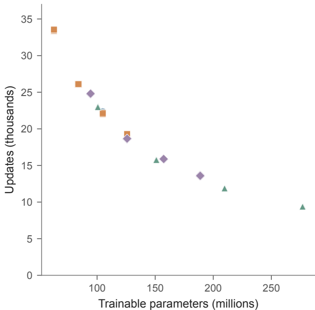
Total updates
