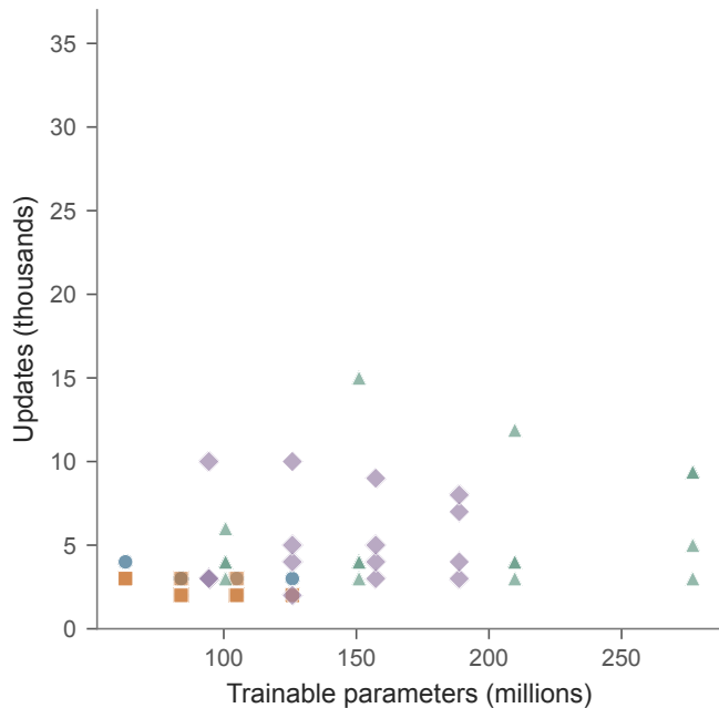
Best-checkpoint update
