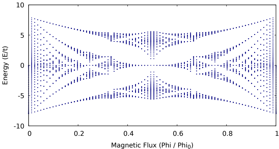
Hofstadter's Butterfly
