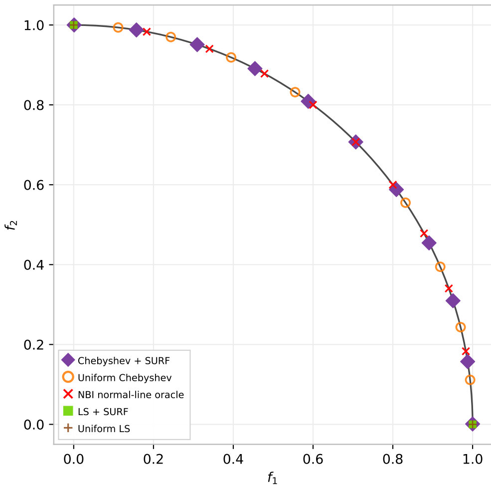
DTLZ2 (M=2): front-oracle spacing diagnostic
