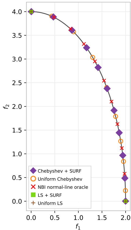
WFG4 (M=2): front-oracle spacing diagnostic
