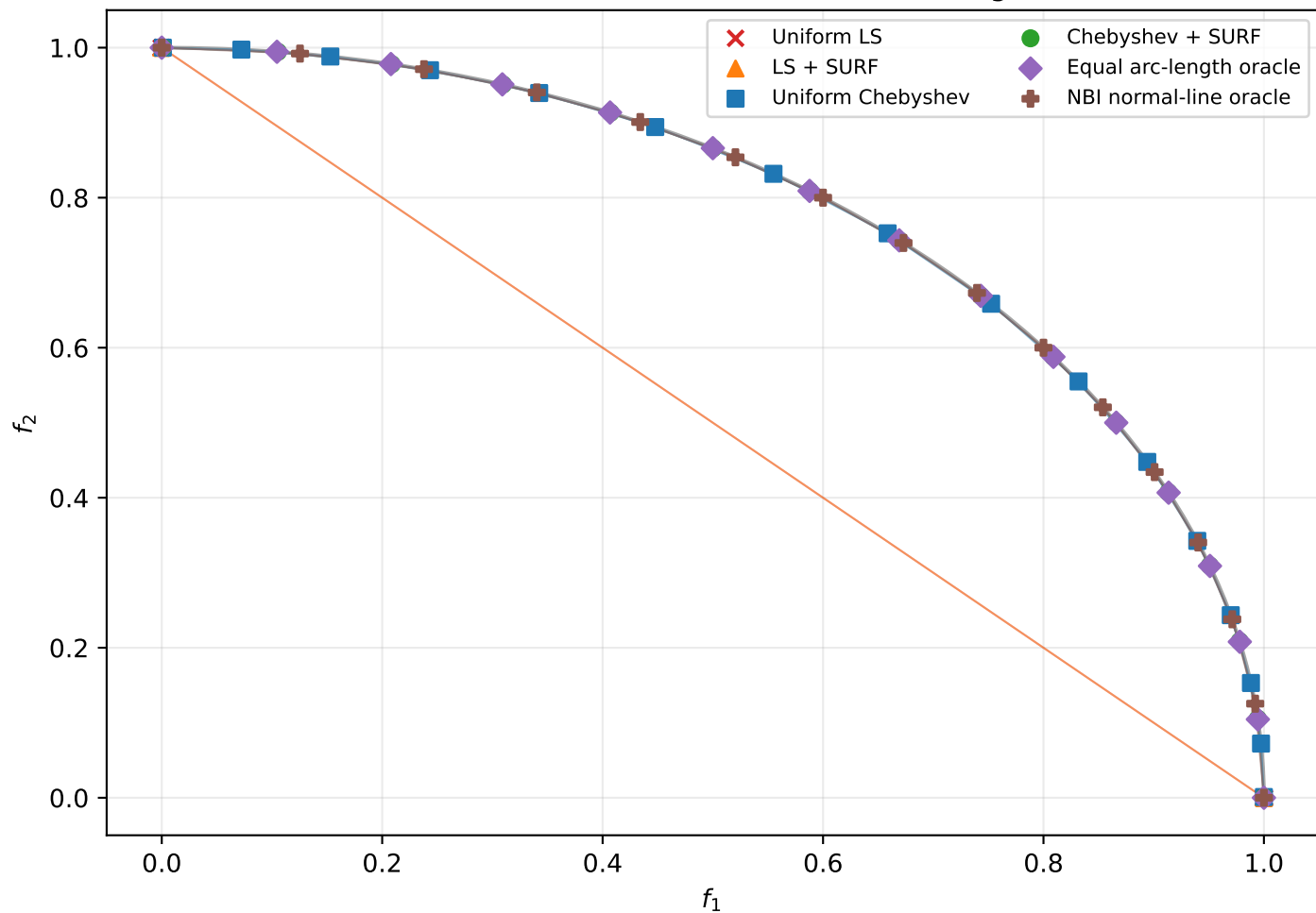
DTLZ2 (M=2): deterministic front-oracle diagnostic
