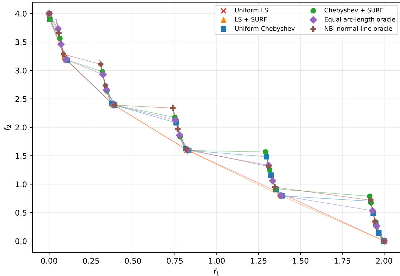
WFG2 (M=2): deterministic front-oracle diagnostic
