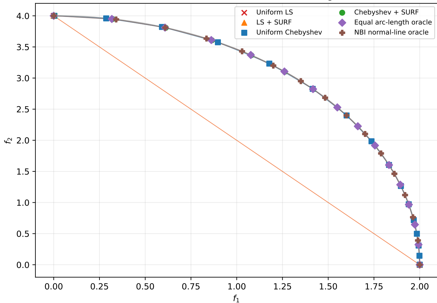
WFG4 (M=2): deterministic front-oracle diagnostic
