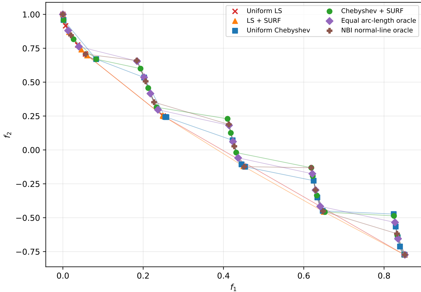
ZDT3: deterministic front-oracle diagnostic
