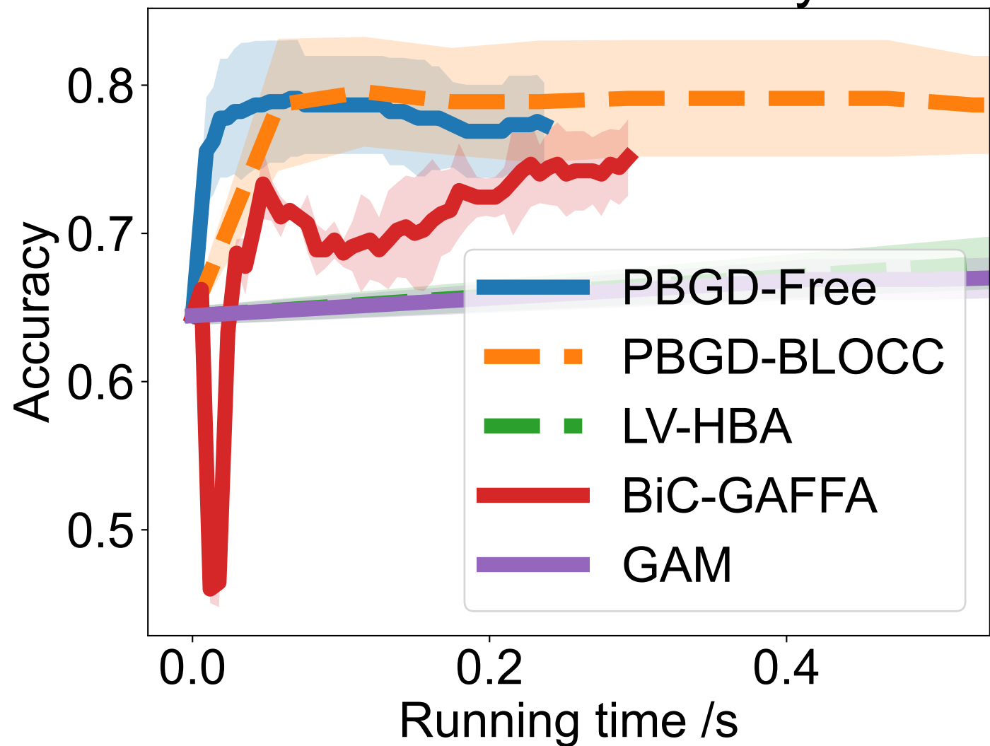
Validation Accuracy
