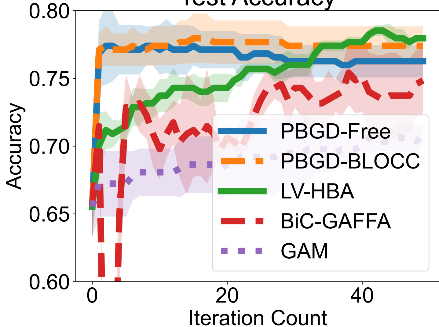
Test Accuracy
