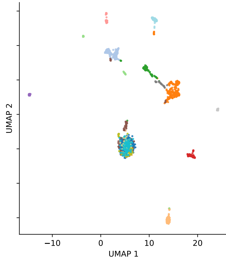
Hisemle (three views) ARI=0.559, NMI=0.686
