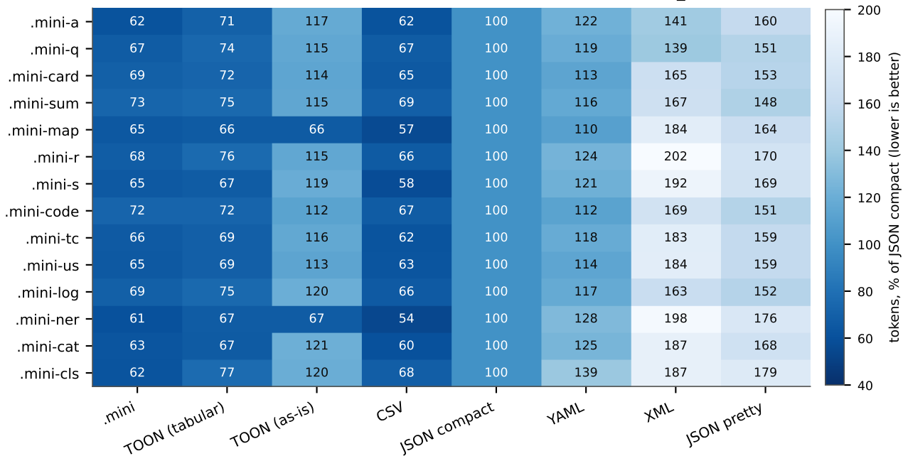
Token cost across 14 domains (n = 12 records, o200k_base)
