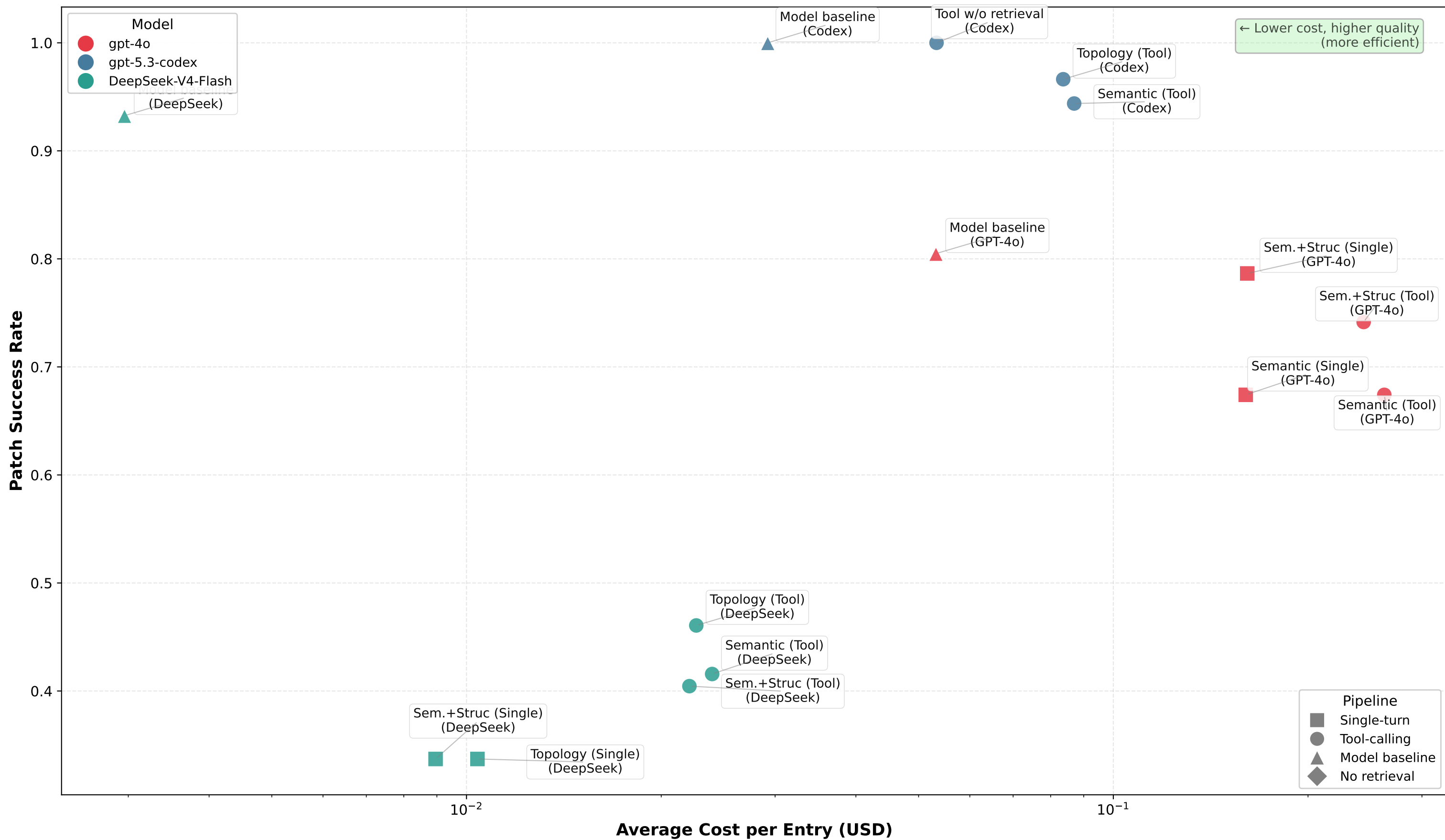
Cost vs. Quality Tradeoff for Vulnerability Patch Generation (CVEFIXES)
