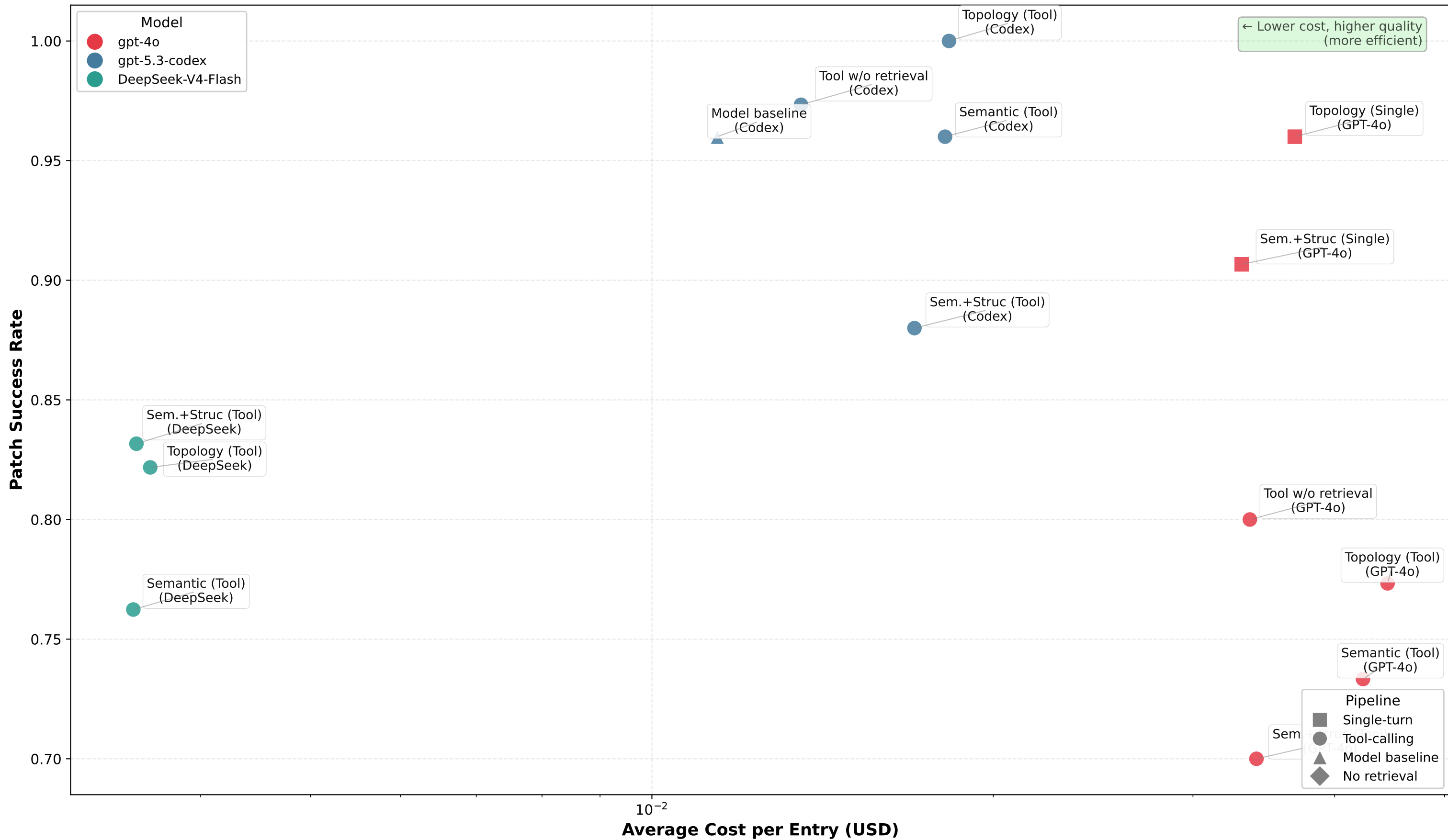
Cost vs. Quality Tradeoff for Vulnerability Patch Generation (AUTOPATCH)
