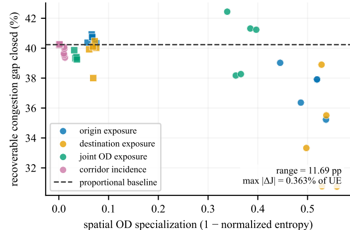
fleet penetration \alpha = 0.5 ; HHI = 0.25
