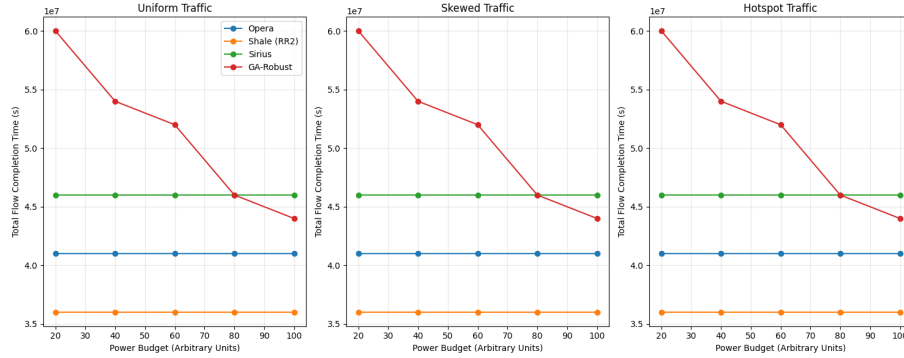
Figure 23: Topology Benchmark: Flow Completion Time vs Power Budget across different traffic models.
