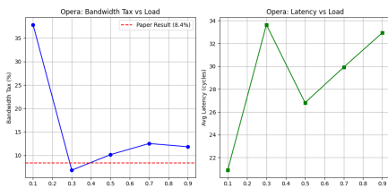
Figure 10: Opera Congestion Tax
