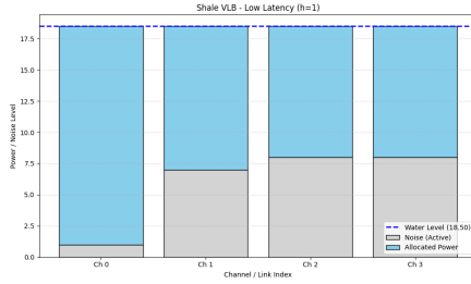
Figure 3: Shale Waterfilling ( h=1 )
