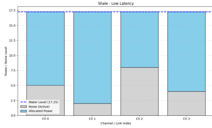
Figure 8: Shale Low Latency Performance
