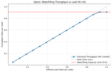
Figure 11: WF Throughput vs Load
