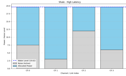
Figure 9: Shale High Latency Performance
