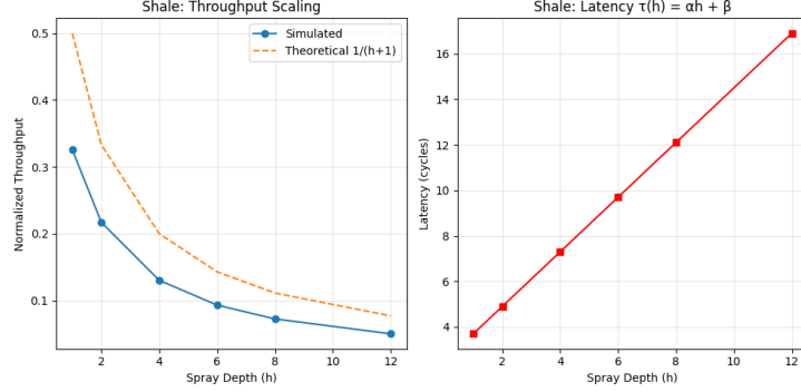
Figure 2: Shale VLB Performance Scaling: Throughput decay vs. theoretical 1/(h+1) (left) and latency regression \tau(h) = \alpha h + \beta (right) for h \in [1, 12] .
