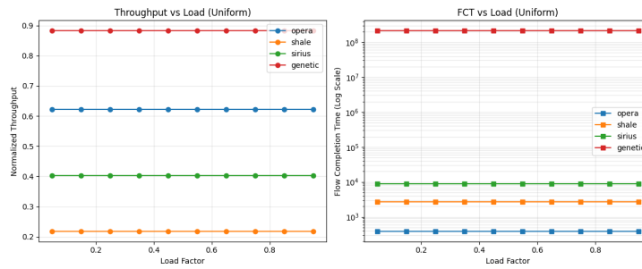
Figure 23: Throughput and FCT vs Load Factor under uniform traffic.
