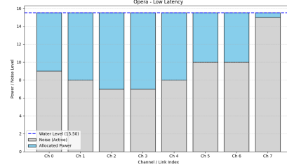
Figure 10: Opera Low Latency Performance
