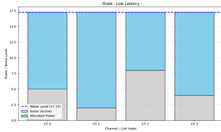
Figure 7: Shale Low Latency Performance
