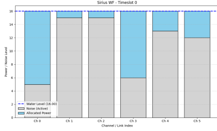
Figure 11: Sirius Waterfilling (TS 0)
