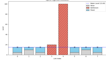
Figure 9: Opera Rigorous Waterfilling
