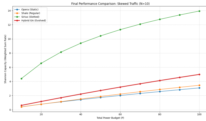
Figure 15: Architecture Comparison under Skewed Traffic using Shannon Capacity
