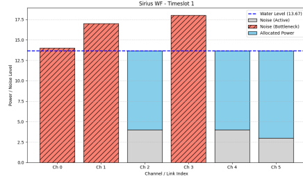
Figure 12: Sirius Waterfilling (TS 1)
