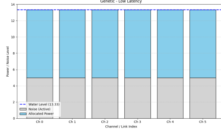
Figure 14: GA Low Latency
