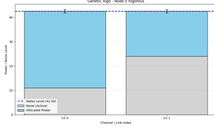
Figure 13: GA Rigorous WF (Node 0)
