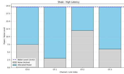
Figure 8: Shale High Latency Performance
