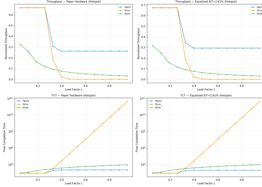
Figure 27: Hotspot traffic: the critical stress test. Under equalized hardware, Sirius still collapses (VLB intermediate saturation [3]) and Shale still degrades (spray convergence on the hot node [2]). Opera maintains the highest throughput because its bulk-circuit scheduling avoids the hotspot [1]. Hardware equalization does not rescue any architecture from its routing-level weakness.
